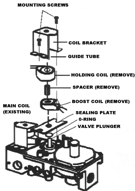
FIG. A. REMOVAL OF BOOST & HOLDING COILS
