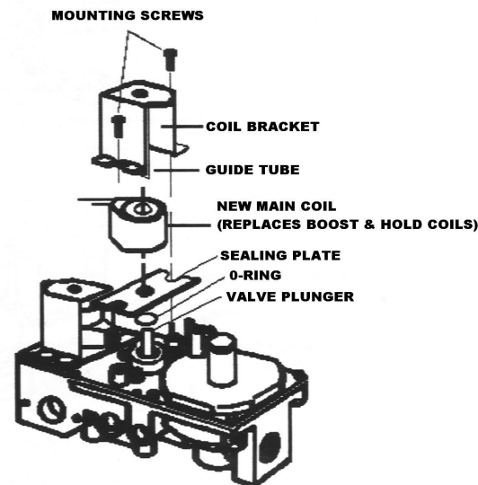
FIG. B. INSTALLING NEW MAIN VALVE COIL
